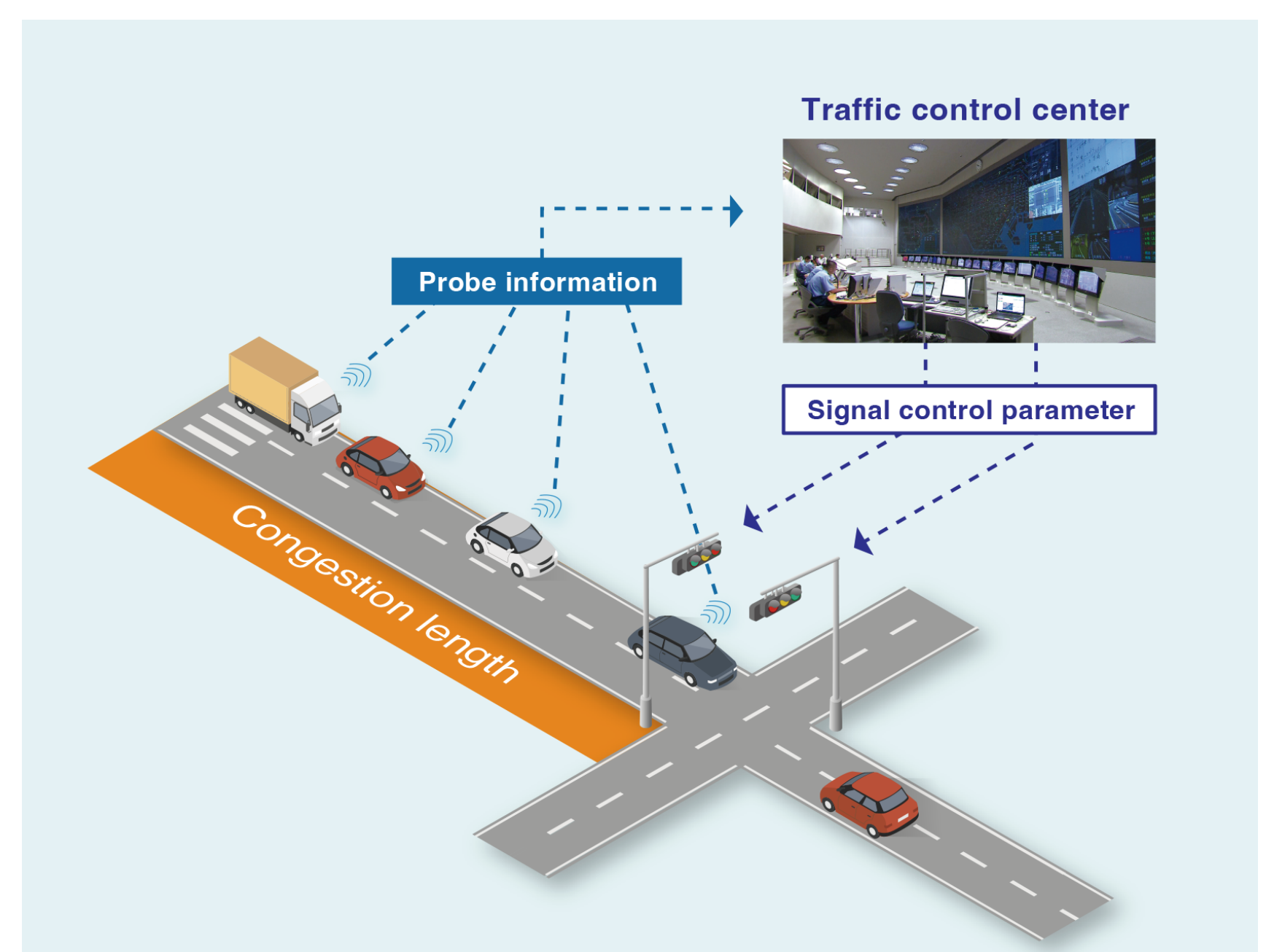
Signal control method using probe information
