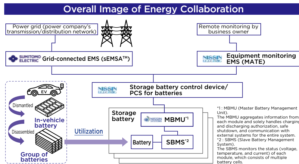
A storage battery system using collected used in-vehicle batteries (illustration)
