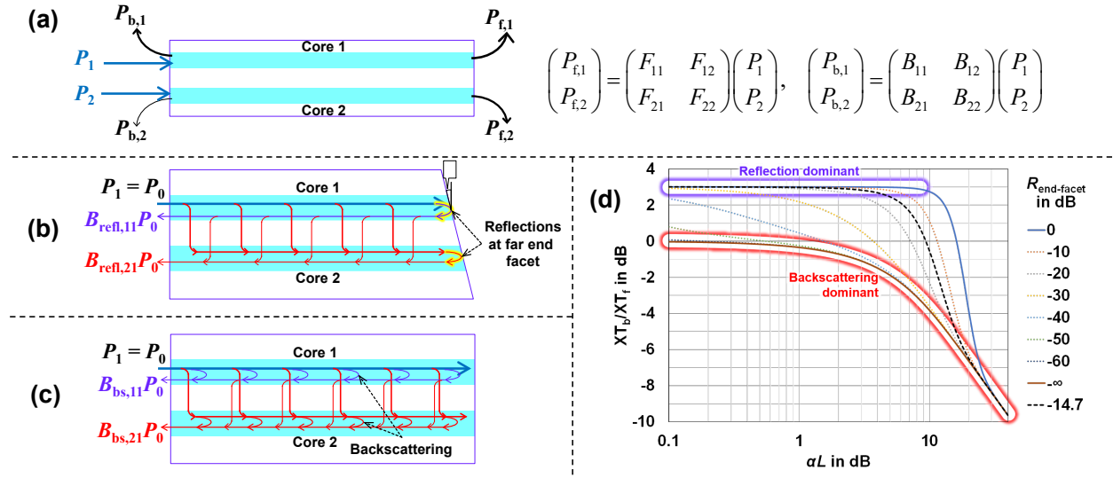
Figure 1. Schematic illustrations depicting (a) forward and backward propagating power transfers for XT definitions, (b) backward propagating power reflected at the non-input end MCF facet with cleave angle \theta , and (c) backward propagating power backscattered by Rayleigh scattering. (d) The ratio of the backward XT to the forward XT vs. the transmission loss \alpha L and the reflectivity R_{\text{end}} , at \lambda = 1.55 \mu\text{m} of an MCF with core design compatible to ITU-T G.657.A1.
