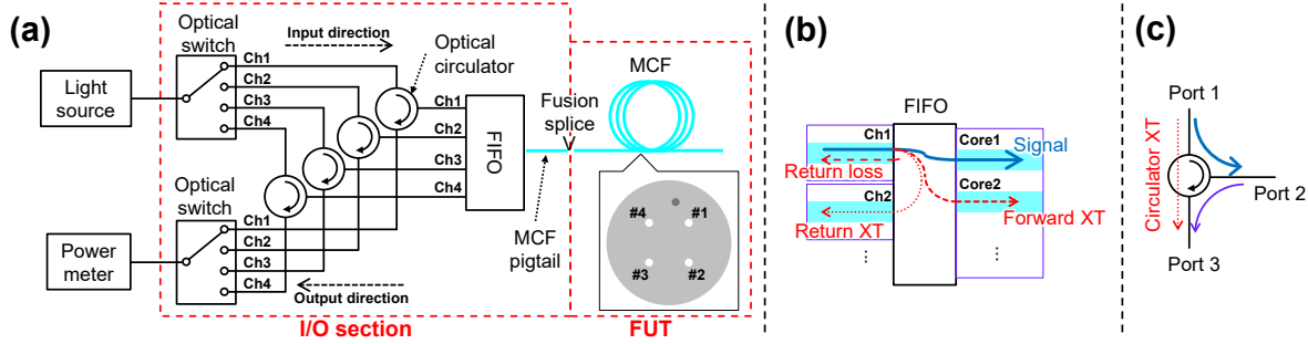
Figure 2. (a) Setup for the single-end XT measurement. (b,c) Noise sources for the measurement in (b) FIFO and (c) circulator.
