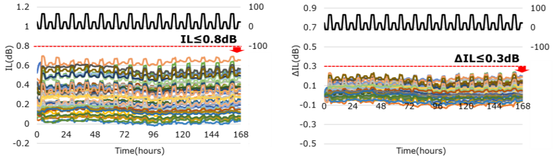
Fig. 7. Results of Humidity Condensation Cycling Test.
