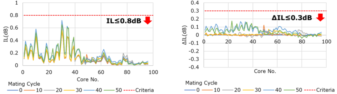
Fig. 6. Results of Durability Test.
