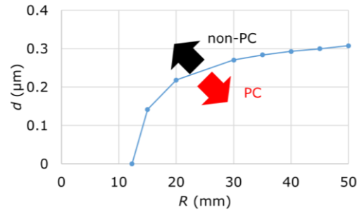
Fig. 4. PC condition of 96-core connector.
