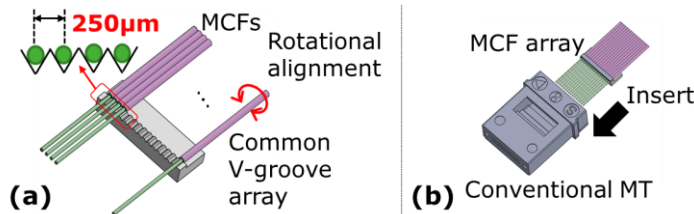
Fig. 1. MT-insertable MCF array method [5] (a) Fabrication of MCF array process (b) Inserting MCF array process.
