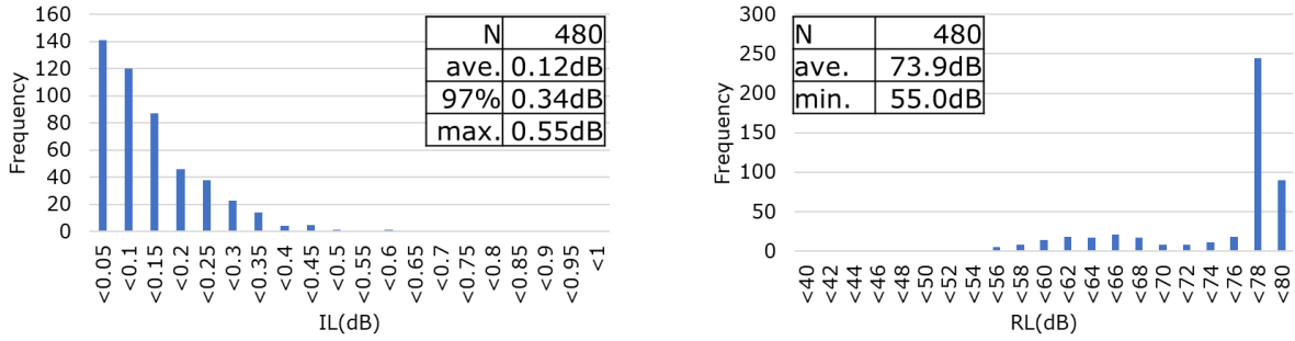
Fig. 5. IL and RL distribution of 5-pairs 96-core MCF-MPO-APC connectors.
