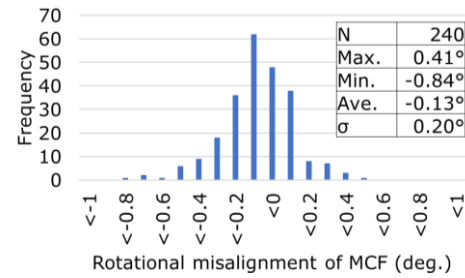
Fig.2. Rotational misalignment of MCF at 10 fabricated 24-MPO connectors.
