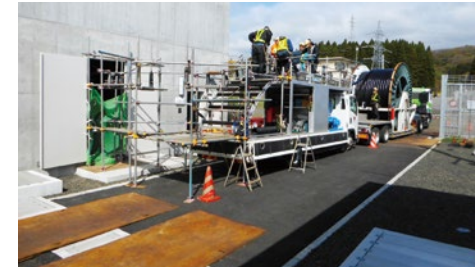
Installation (on the Hokkaido side: Yoshioka cable head (draw-in port))
