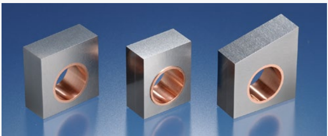
Tungsten monoblock: A product with a size of approximately 30 mm x 30 mm x 10 mm, which is made by bonding tungsten material suitable for fusion reactors and oxygen-free copper by using a special bonding method. This is skewed by a copper alloy cooling pipe to form a unit.
