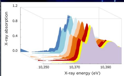
In-situ X-ray absorption spectroscopy measurements using synchrotron radiation for the interface state between an insulation film and semiconductor when the GaN-HEMT is in operation
