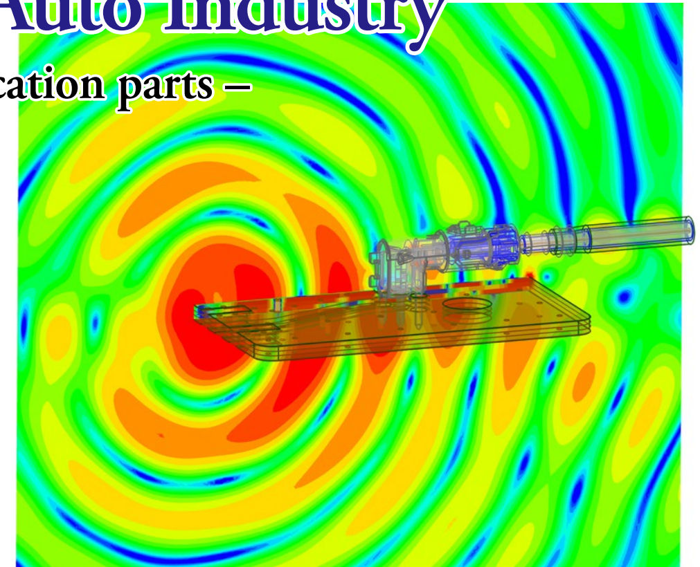
This electromagnetic noise radiation chart based on high-frequency CAE shows the strength of waves during electromagnetic radiation at the connector (red: strong). The waves propagate in varying intensity.
