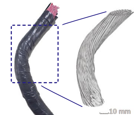
The appearance of the cable and X-ray CT 3D image, which offers findings required for CAE
