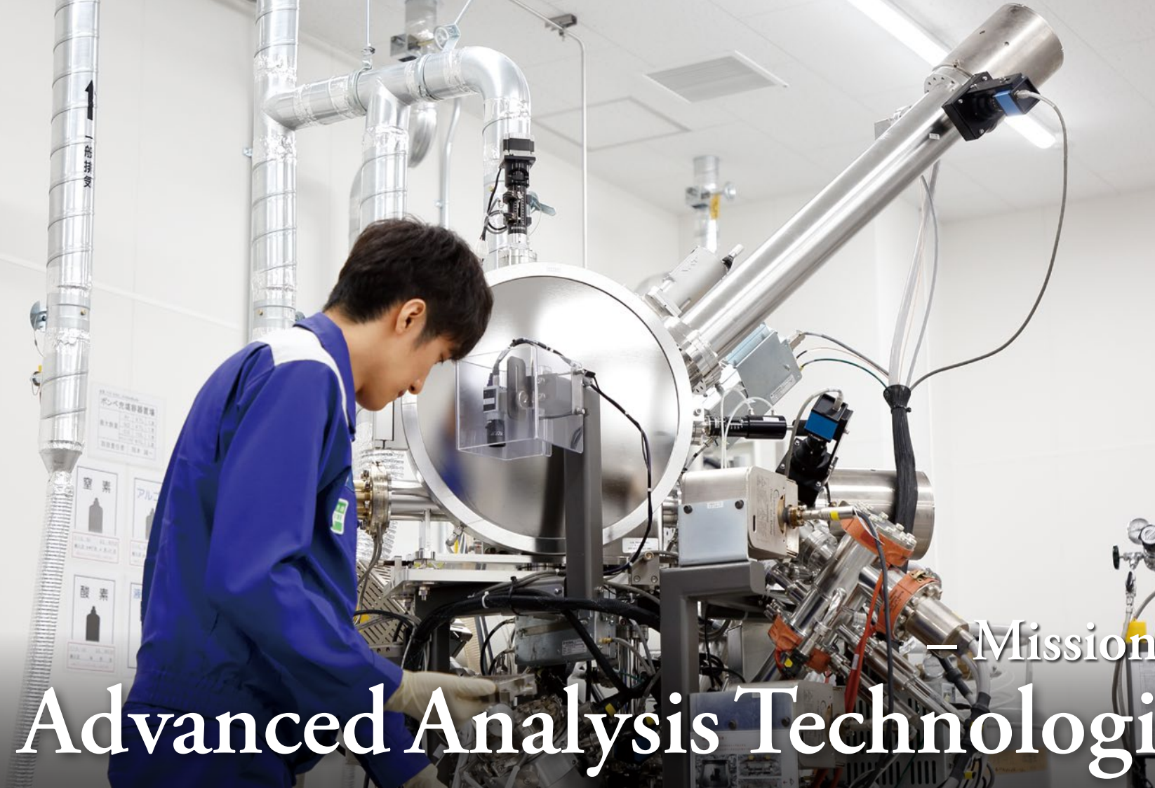
Time-of-Flight Secondary Ion Mass Spectrometry (ToF-SIMS) achieves high-sensitivity surface analysis of elements and structures of chemical species.
