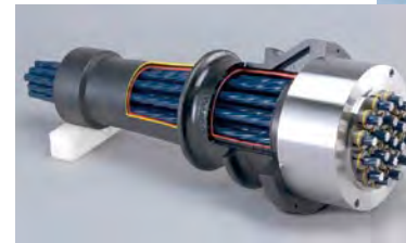
Pre-grouted prestressing steel strand
