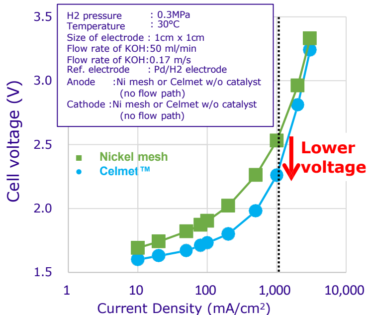
Polarization of Curves with Celmet™ and Ni Mesh as Electrodes
