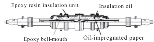
Fig. 9. Transition joint for Kitahon HVDC Link
