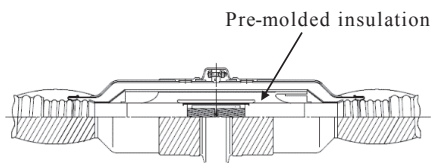
Fig. 12. Pre-molded one piece joint
