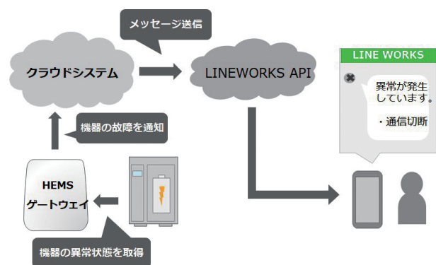
図7 故障検知
