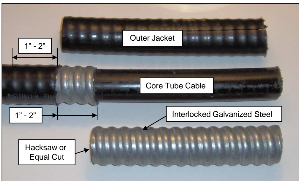
Figure 5 Interlocked Galvanized Steel Tube Cable Outer Jacket and Armor Removed
