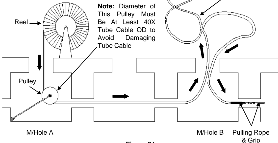
Figure 24 Section Pulling Method
