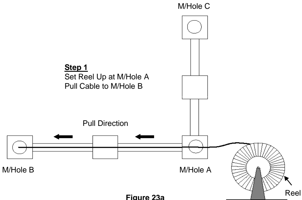
Figure 23a Bi-Direction Pulling Method
