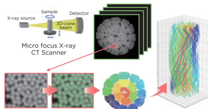
CT images of Electric wire cable(173x19=3287cables), and the quantification result of these image
