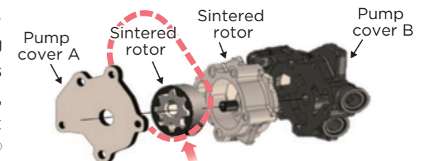
FEX ® coated on both ends of a gear rotor.
